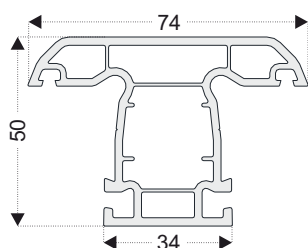
PRO533 Mullion Profile
