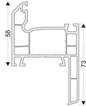
PRO81 Renovation Frame Prf.
