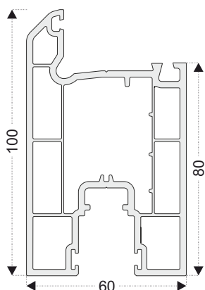
PRO24 Sliding Door Sash Profile
