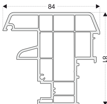
PRO8622 French Casement Mullion Prf.
