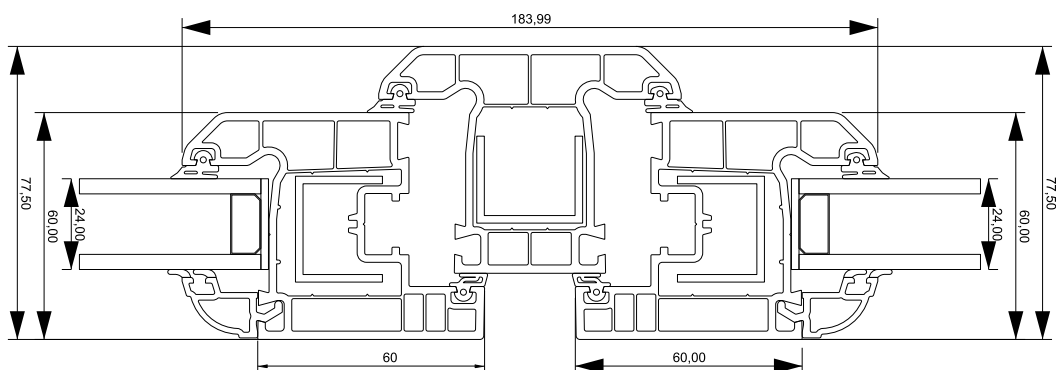
Sash - Mullon - Sash Connection Section
