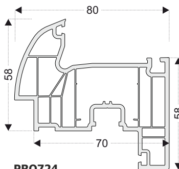
PRO724 Drain Sash Profile (7 Chambers)
