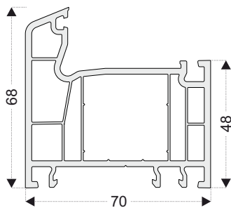
PRO710 Frame Profile - 48mm
