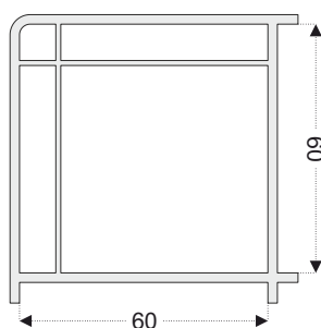
PRO36 Box Profile - 60x60mm (60mm Series)
