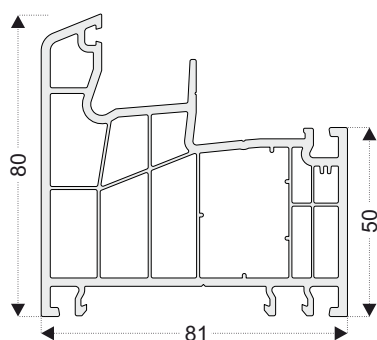
PRO8601 Frame Profile
