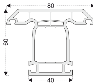
PRO003 Mullion Profile
