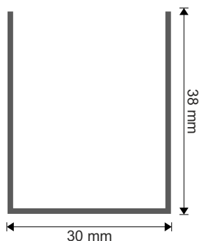
38 x 30 x 38 PRO10, PRO715 PRO716
