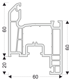
PRO002 Sash Profile
