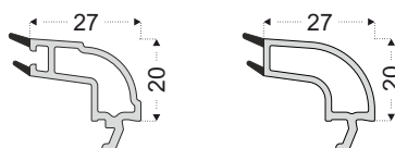
PRO701 20-22 mm Double Glass G.Bead
