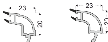
PRO702 24-26 mm Double Glass G.Bead
