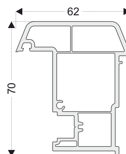
PRO717 French Casement Mullion Prf.
