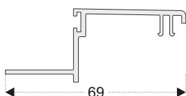
PRO28 Double Sliding Frame Trim Profile (Alum.)
