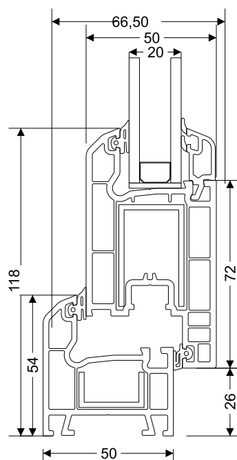
Frame - Inward Opening Door Sash Connection Section
