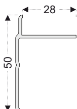
PRO35 T Trim Profile (60mm Series)
