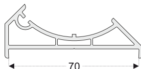
PRO331 Corner Profile - 70mm
