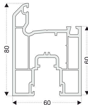
PRO21 Sliding Door Sash Profile
