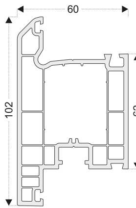
PRO10 Outward Door Profile
