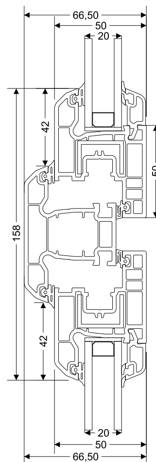
Sash - Mullion - Sash Connection Section
