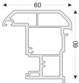
PRO12 French Casement Mullion Prf.
