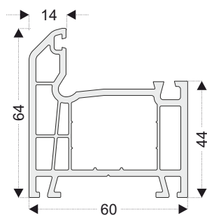
PRO001 Frame Profile
