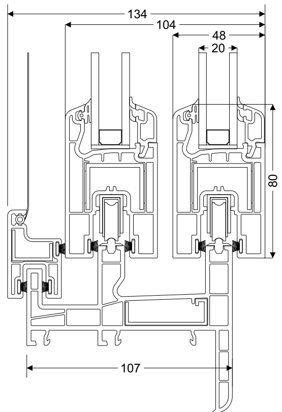
Double Sliding Frame - Sliding Sash with Flynet
