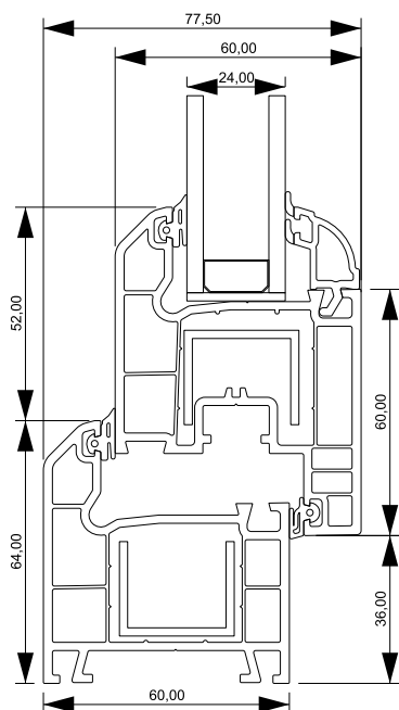
Frame - Sash Connection Section
